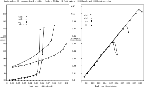
Figure 5: Performance comparison in 16x16x16 meshes.
