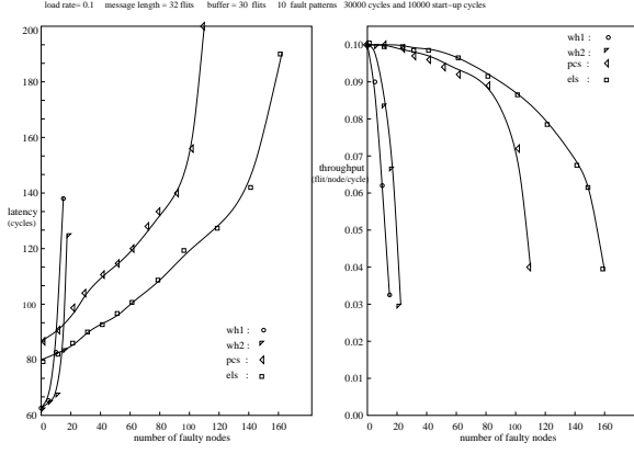
Figure 4: Performance comparison in 8x8x8 meshes with fixed load rate.
