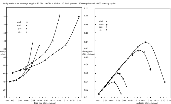
Figure 3: Performance comparison with PCS and the wormhole routing techniques in 8x8x8 meshes.
