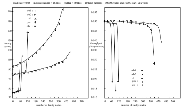
Figure 6: Performance comparison in 16x16x16 meshes with fixed load rate.
