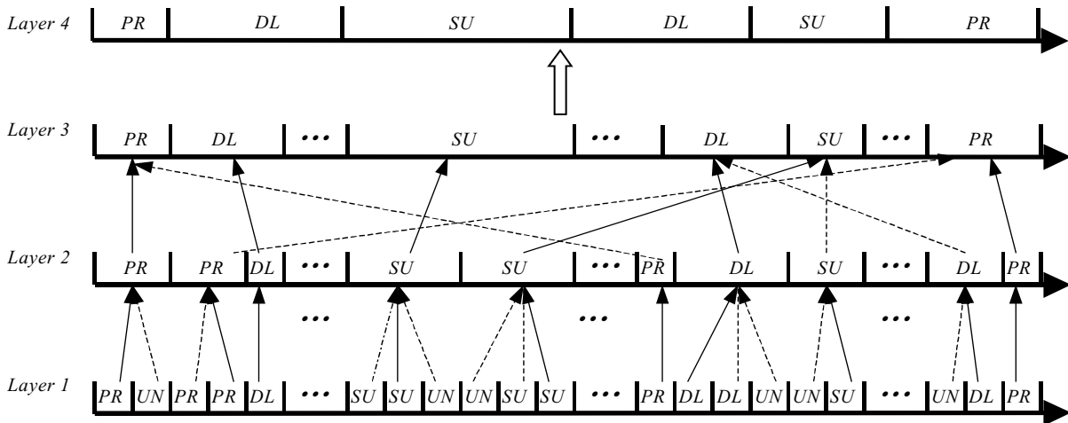
Fig. 11. Hierarchical video summarization strategy. ( PR , DL , SU and UN represent presentation, dialog, surgery, and unknown events respectively; the solid line indicates that this group is selected as the representative group of the newly generated unit)
