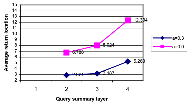
Fig. 16. Video retrieval results with summaries at different levels
