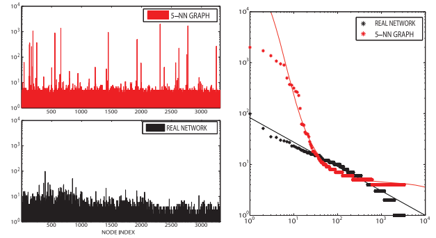
Fig. 2. The difference between real-world network topology structures versus synthetic k -NN graph (affinity graph) on CiteSeer data set. The left figures show logarithmic scale node degrees ( y -axis) w.r.t. nodes indexed by the x -axis. The lower panel shows node degrees for genuine CiteSeer networks and the upper panel shows node degrees for the 5-NN graph. Results show that instances (nodes) with high degrees are different in real network versus the 5-NN graph. The right figure shows that real network follows power-law distribution whereas the 5-NN graph follows geometric distribution, where the colored lines show the fitted functions. The results confirm that a k -NN graph does not capture real-world network distributions.
