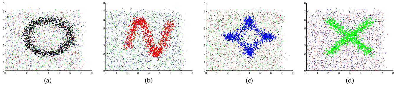
Fig. 5. The genuine clusters of the synthetic network (best viewed in color). (a) The distribution of features 1 and 2 is a circle. (b) The distribution of features 3 and 4 is a sine function. (c) The distribution of features 5 and 6 is a star function. (d) The distribution of features 7 and 8 is a absolute value function.
