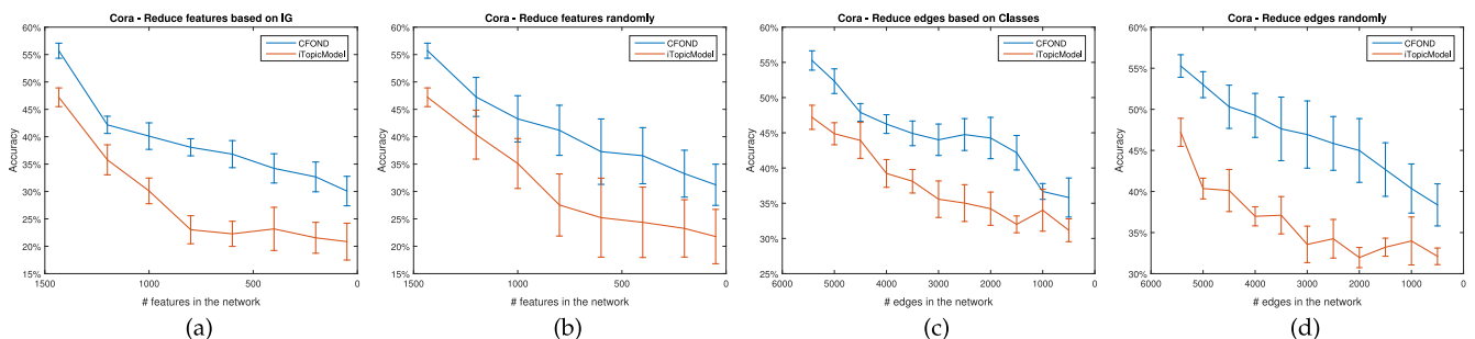
Fig. 10. Case study of CFOND versus iTopicModel on networks with various degree of consistency between node content and topology structures (a) and (b), and networks with different degree of edge density (c) and (d).
