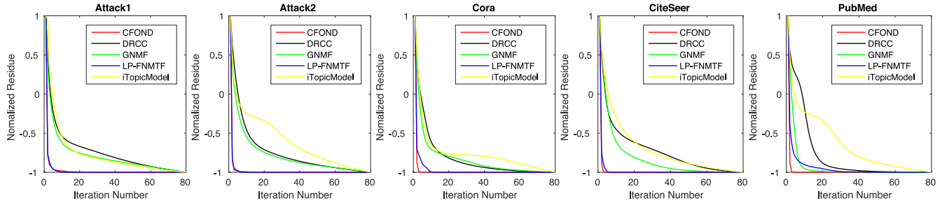
Fig. 8. Convergence comparisons of different co-clustering methods on real-world data sets. The x -axis denotes the number of iterations, and the y -axis denotes the normalized residue of the objective function.
