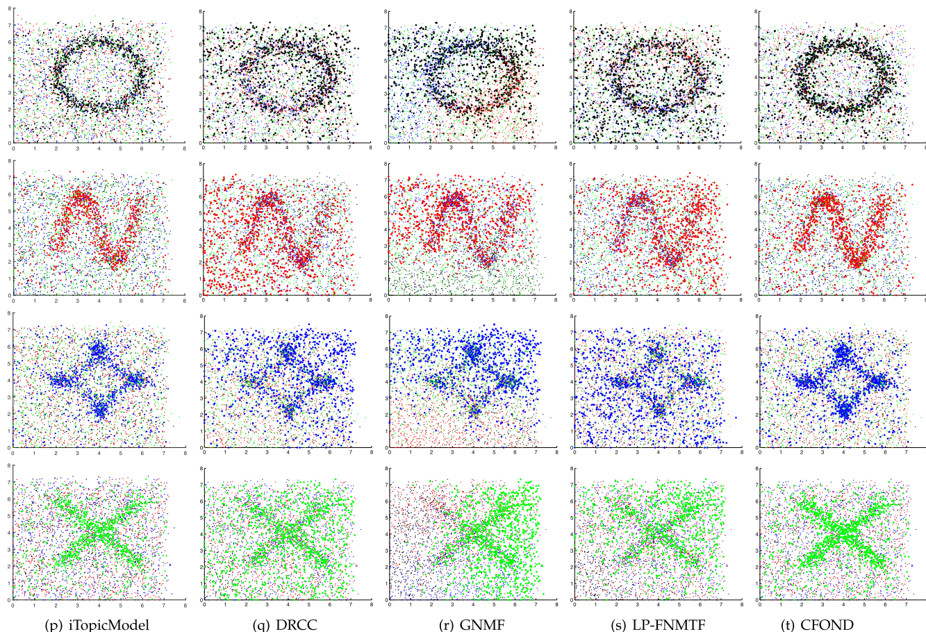
Fig. 6. Co-clustering results from iTopicModel, DRCC, GNMF, LP-FNMTF, and CFOND on the synthetic network. The genuine clusters are a circle function, a sine function, a star function, and an absolute value function showing in Fig. 5. Each column shows co-clustering results of one method.
