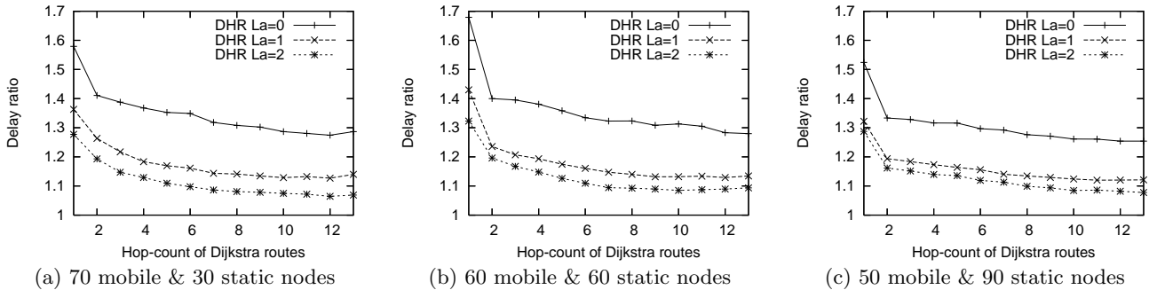
Figure 12: The ratio of the delay of the DHR (with different L_a s) routes to that of the Dijkstra routes in networks of different numbers of mobile nodes and static nodes.
