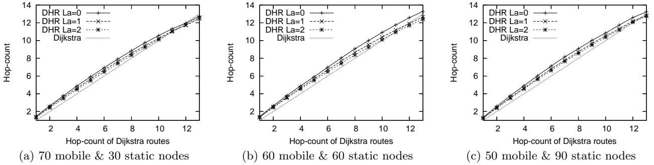
Figure 9: Hop-count of DHR (with different L_a s) routes compared with that of the Dijkstra routes in networks of different numbers of mobile nodes and static nodes.
