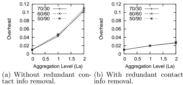
Figure 14: Storage/communication overhead.
