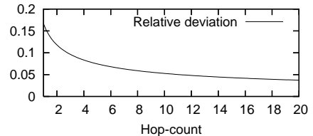
Figure 6: The inaccuracy of the time-invariant delay represented by the relative deviation \frac{\sigma_n}{\mu_n} .
