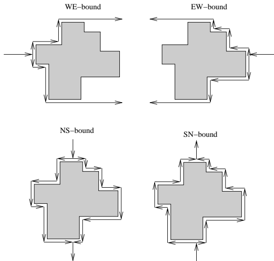
Figure 1. Routing of messages around disabled regions.
