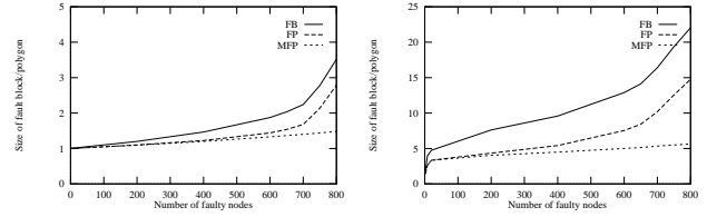
Figure 10. Average size of FB, FP, and MFP: (a) the random fault distribution model and (b) under the clustered fault distribution model.
