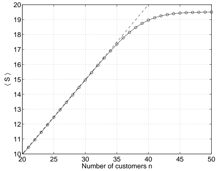
Figure 2: The expected quantity of resource being allocated \langle S \rangle against the number of customers n for \bar{k} = 20 .
