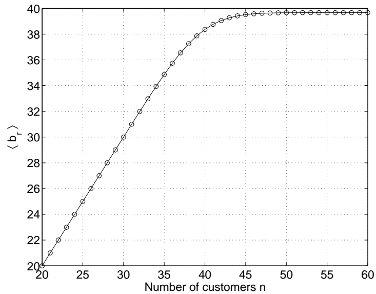
Figure 3: The expected number of clients being allocated \langle b_r \rangle with resource against the number of customers n for \bar{k} = 20 .
