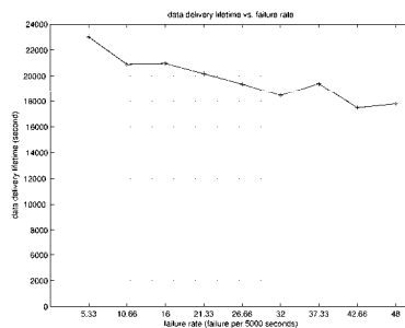
Figure 13. Data Delivery Lifetime with Failures
