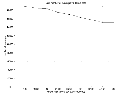
Figure 14. Average Total Wakeup Count for Failure Rates
