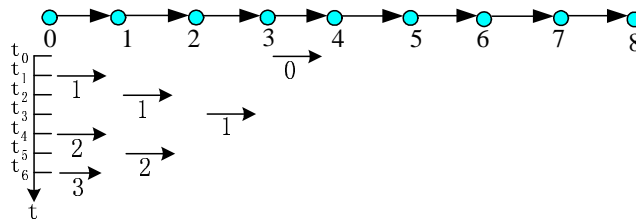
Fig. 8. The packet scheduling when congestion occurs at node 4. The congestion can result from the interference or contention from any crossing flow such that node 4 can not grab the channel in time.
