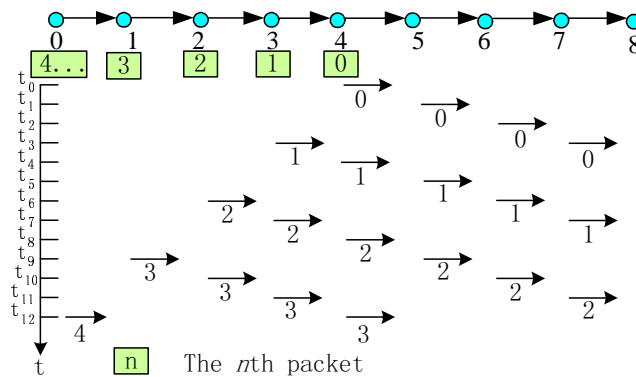
Fig. 9. The packet scheduling after eliminating the congestion at node 4. After the backward-pressure scheduling takes effect, the upstream nodes of this flow and all other crossing flows yield the transmission opportunity to the congested node. Thus node 4 can quickly forward the backlogged packets and hence the congestion is eliminated.
