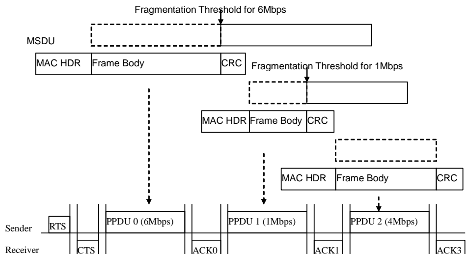
Fig. 10. Dynamic fragmentation process and the timeline of data transmission
