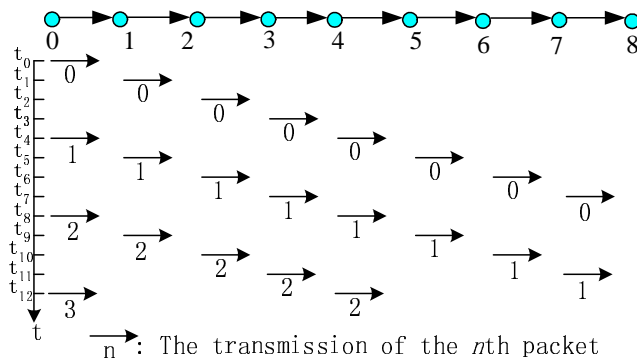
Fig. 6. Optimum packet scheduling for chain topology. To simplify the illustration how our scheme work, we use chain topology in this figure and following ones, which is conceptually the same with any random multihop path in the mobile ad hoc networks.
