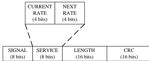
Fig. 11. Physical layer header format in the proposed protocol
