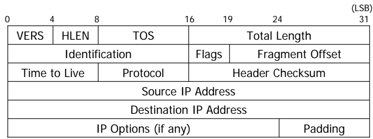
Format of an IP datagram header
