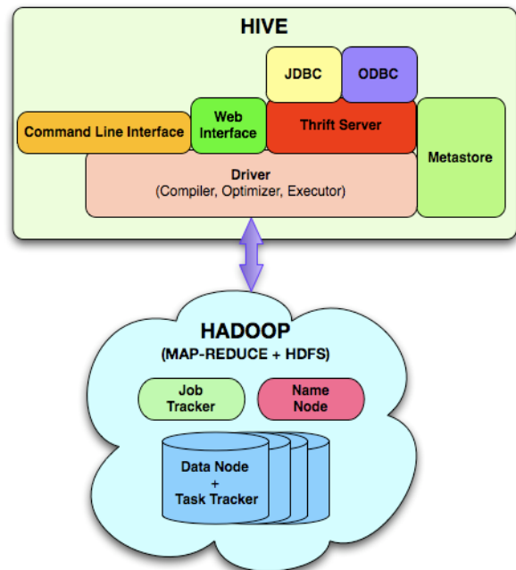
Figure 2: Hive System Architecture
