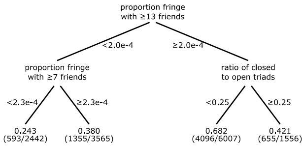
Figure 5: The top two levels of decision tree splits for predicting community growth in LiveJournal.
