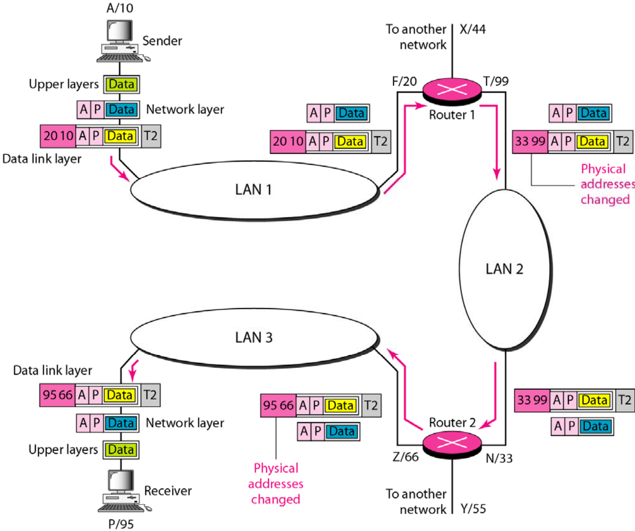
Figure 2.20 IP addresses
