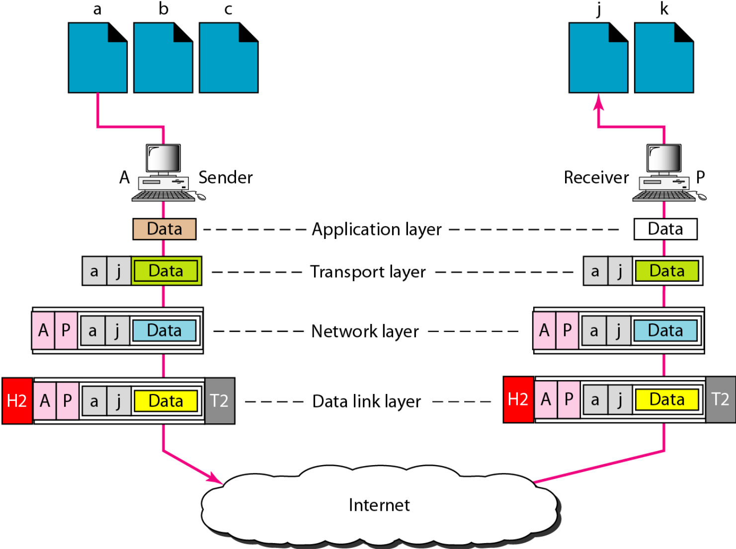
Figure 2.21 Port addresses
